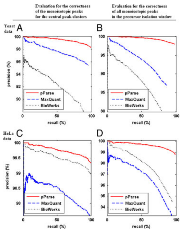
Figure 2. Evaluation for the correctness of monoisotopic peaks. Two evaluation approaches are designed in the text: (i) evaluation for the correctness of the monoisotopic peaks for the central peak clusters and (ii) evaluation for the correctness of all monoisotopic peaks in the precursor isolation window. Points (A) and (B) are the precision recall curves for the Yeast data, while (C) and (D) are the precision recall curves for the HeLa data. In four cases pParse is the most sensitive and the sensitivity on all identified monoisotopic peaks reaches more than 98%.
