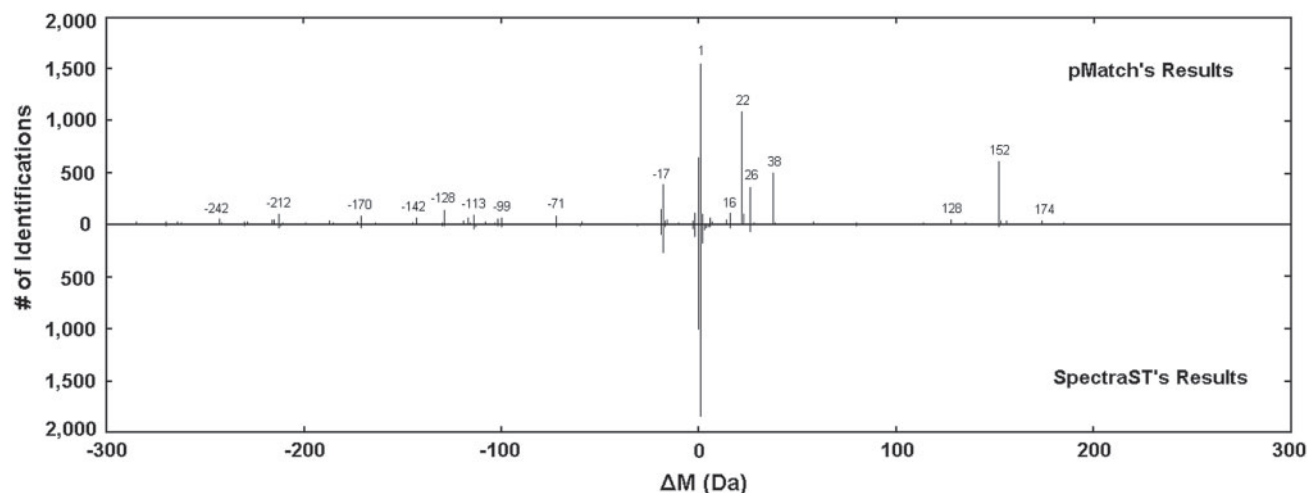
Fig. 4. Histograms of \Delta M detected by pMatch (top) and SpectraST (bottom). The intensive peaks are annotated by their \Delta M values in integer accuracy.
